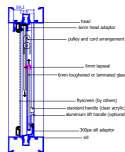
Vertical 2 Pane Section
