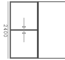
Double Hung with Fixed
