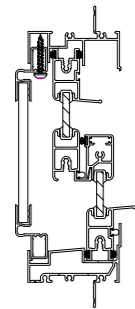
Vertical Section
