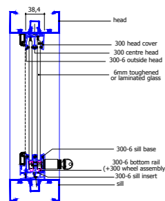
Horizontal 2 Pane Section
